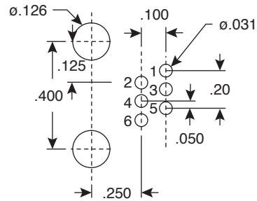
PCB Hole Layout
