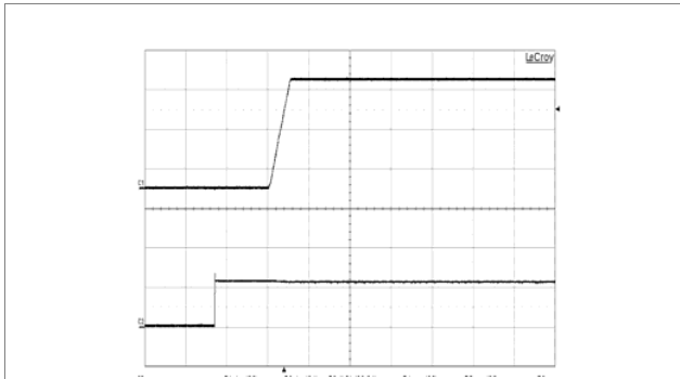
Start-up enabled by connecting V_i at: T_{P1} = +25^\circ\text{C} , V_i = 12\text{ V} , I_o = 18\text{ A} resistive load. Top trace: output voltage (2 V/div.). Bottom trace: input voltage (10 V/div.). Time scale: (20 ns/div.).
