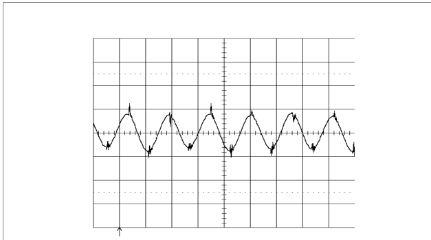
Output voltage ripple at: T_{P1} = +25^\circ\text{C} , V_i = 12\text{ V} , I_o = 18\text{ A} resistive load. Trace: output voltage (20 mV/div.). Time scale: (2 \mu\text{s} /div.).
