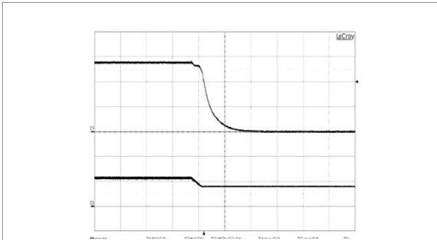
Shut-down enabled by disconnecting V_i at: T_{P1} = +25^\circ\text{C} , V_i = 12\text{ V} , I_o = 18\text{ A} resistive load. Top trace: output voltage (2 V/div.). Bottom trace: input voltage (10 V/div.). Time scale: (0.5 ms/div.).
