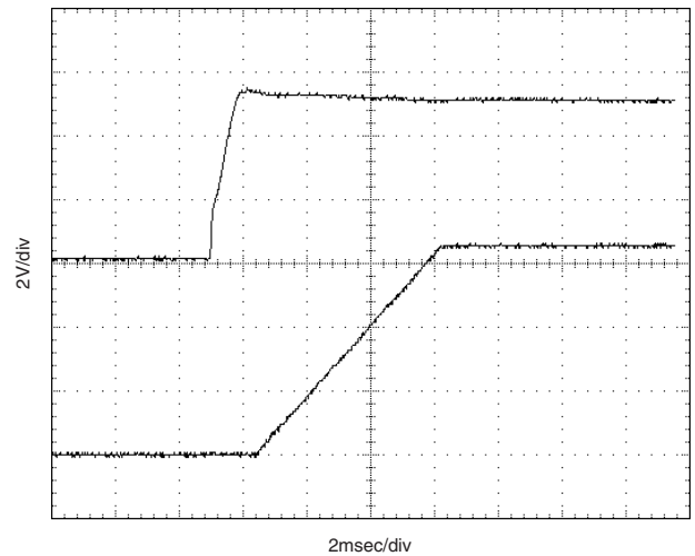
Power-Up From V IN (V IN = 5V, V OUT = 3.3V/10A, C IN = 220μF, No External C OUT )
