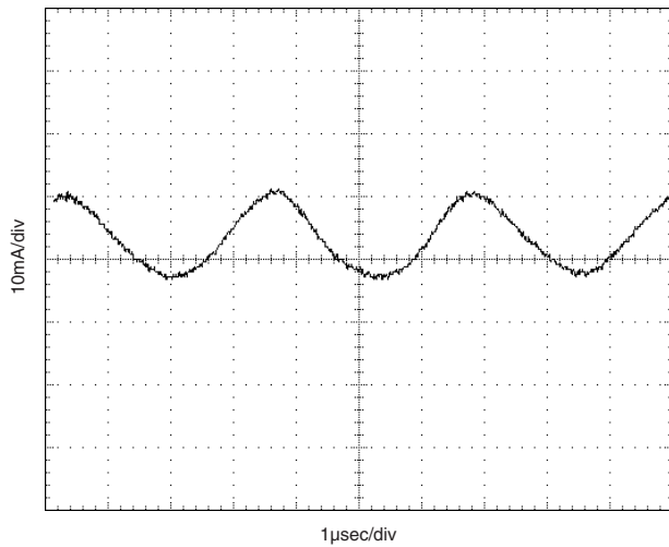
Input Reflected Ripple Current (V IN = 5V, V OUT = 3.3V/10A, C IN = 220μF, No External C OUT )
