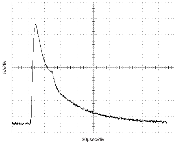
Input Inrush Current (V IN = 5V, 4300μF as Input Switch )
