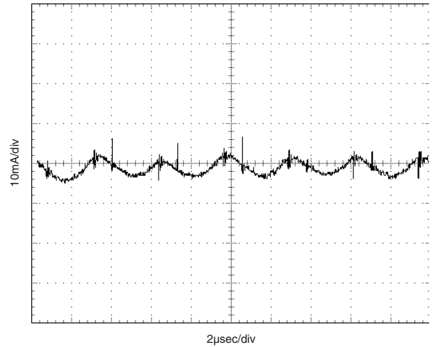
Input Reflected Ripple Current (V IN = 5V, V OUT = 3.3V/10A, Input Filter = 220μF/12μH/33μF, C OUT = NA)
