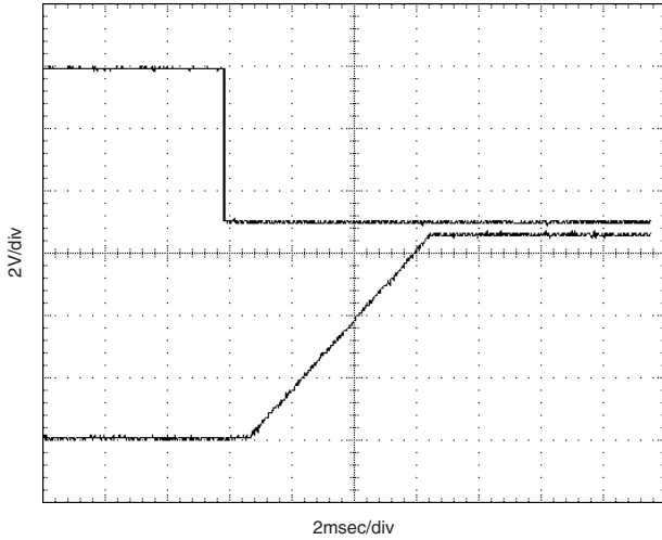
Power-Up From Enable
