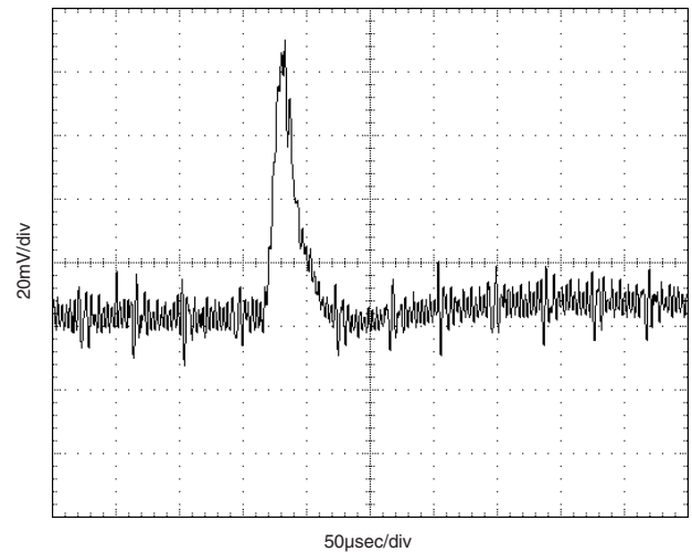
Dynamic Load Response
