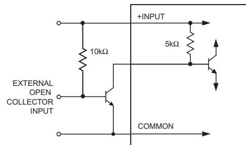
External Input Open: On/Off pin Low = DC/DC converter Off External Input Low: On/Off pin High = DC/DC converter On
