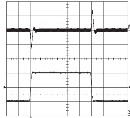
Output voltage response to load current step-change (1.05-3.15-1.05A) at T_{Pcb}=+25 °C, V_{in}=27 V. Top trace: output voltage (200mV/div.). Bottom trace: load current (1.0 A/div.). Time scale: 0.1 ms/div.
