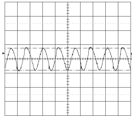
Output voltage ripple (50mV/div.) at T_{Pcb}=+25 °C, V_{in}=27 V, I_o=4.2 A resistive load with C=10 \mu F tantalum and 0.1 \mu F ceramic capacitors. Band width=20MHz. Time scale: 2 \mu s / div.
