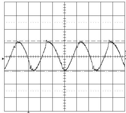
Output voltage ripple (50mV/div.) at T_{Pcb}=+25 °C, V_{in}=27 V, I_o=3.33 A resistive load with C=10 \mu F tantalum and 0.1 \mu F ceramic capacitors. Band width=20MHz. Time scale: 1 \mu s / div.
