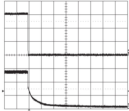
Turn-off at I_o=3.33 A resistive load at T_{Pcb}=+25 °C, V_{in}=27 V. Turn-off enabled by disconnecting V_{in} . Top trace: output voltage (10 V/div.). Bottom trace: input voltage (5 V/div.). Time scale: 10 ms/div.
