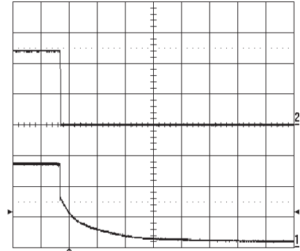
Turn-off at I_o=4.2 A resistive load at T_{Pcb}=+25 °C, V_{in}=27 V. Turn-off enabled by disconnecting V_{in} . Top trace: output voltage (10 V/div.). Bottom trace: input voltage (5 V/div.). Time scale: 10 ms/div.
