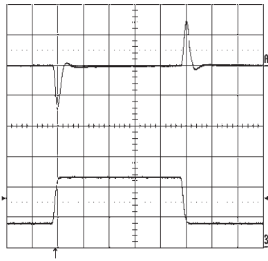
Output voltage response to load current step-change (3.75-11.25-3.75 A) at T_{Pcb}=+25\text{ }^{\circ}C , V_{in}=27\text{ V} . Top trace: output voltage (200mV/div.). Bottom trace: load current (5 A/div.) Time scale: 0.1 ms/div.
