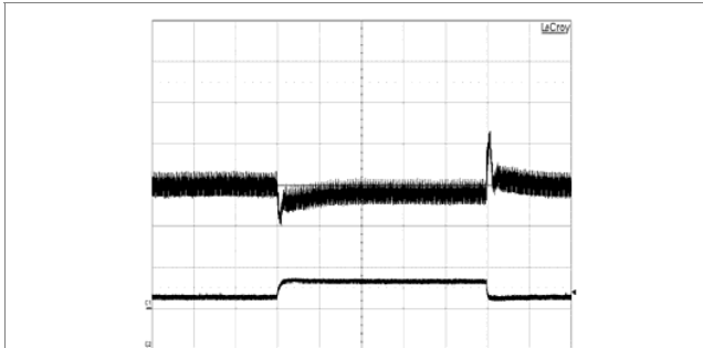
Output voltage response to load current step-change (7.5-22.5-7.5 A) at: T_{ref} = +25^\circ\text{C} , V_i = 53\text{ V} . Top trace: output voltage (100 mV/div.). Bottom trace: load current (30 A/div.). Time scale: (0.1 ms/div.).
