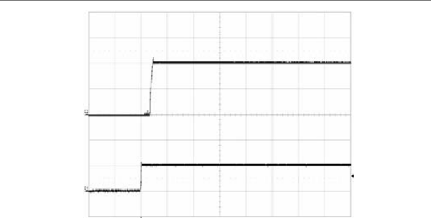
Start-up enabled by connecting V_i at: T_{ref} = +25^\circ\text{C} , V_i = 53\text{ V} , I_o = 30\text{ A} resistive load. Top trace: output voltage (0.5 V/div.). Bottom trace: input voltage (50 V/div.). Time scale: (5 ms/div.).
