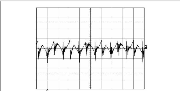
Output voltage ripple at: T_{ref} = +25^\circ\text{C} , V_i = 53\text{ V} , I_o = 30\text{ A} resistive load. Trace: output voltage (20 mV/div.). Time scale: (2 \mu\text{s} /div.).
