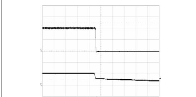
Shut-down enabled by disconnecting V_i at: T_{ref} = +25^\circ\text{C} , V_i = 53\text{ V} , I_o = 30\text{ A} resistive load. Top trace: output voltage (0.5 V/div.). Bottom trace: input voltage (50 V/div.). Time scale: (0.5 ms/div.).
