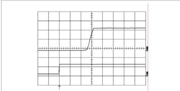
Start-up enabled by connecting V_i at: T_{ref} = +25^{\circ}\text{C} , I_O = 10\text{ A} resistive load, V_i = 12.0\text{ V} . Top trace: output voltage (1.0 V/div.), Bottom trace: input voltage (10 V/div.). Time scale: 5 ms/div.
