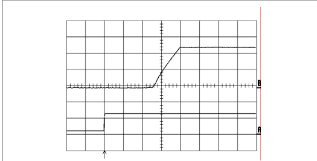
Start-up enabled by connecting V_i at: T_{ref} = +25^{\circ}\text{C} , I_O = 10\text{ A} resistive load, V_i = 12.0\text{ V} . Top trace: output voltage (2.0 V/div.). Bottom trace: input voltage (10 V/div.). Time scale: 5 ms/div.
