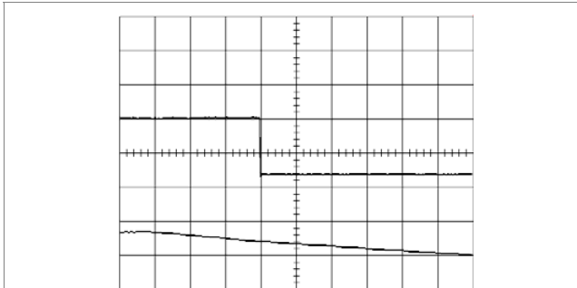
Shut-down enabled by disconnecting V_i at: T_{ref} = +25^{\circ}\text{C} , I_O = 10\text{ A} resistive load, V_i = 12.0\text{ V} . Top trace: output voltage (2.0 V/div.). Bottom trace: input voltage (10 V/div.). Time scale: 5.0 ms/div.
