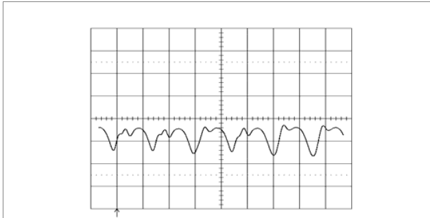
Output voltage ripple (20mV/div.) at: T_{ref} = +25^{\circ}\text{C} , I_O = 10\text{ A} resistive load, V_i = 12.0\text{ V} . Time scale: 2 \mu\text{s} /div. See the filter in the Output ripple and noise section (EMC Specification).
