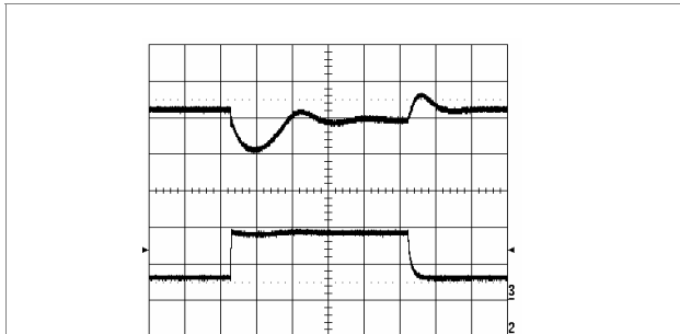
Output voltage response to load current step-change (0.3-0.9-0.3 A) at: T_{ref} = +25^{\circ}\text{C} , V_i = 53\text{ V} . Top trace: output voltage (200mV/div.). Bottom trace: load current (0.5 A/div.). Time scale: 0.1 ms/div.
