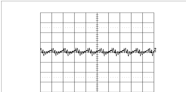
Output voltage ripple (10mV/div.) at: T_{ref} = +25^{\circ}\text{C} , I_o = 1.2\text{ A} resistive load, V_i = 53\text{ V} . Time scale: 2 μs/div. See the filter in the Output ripple and noise section (EMC Specification).
