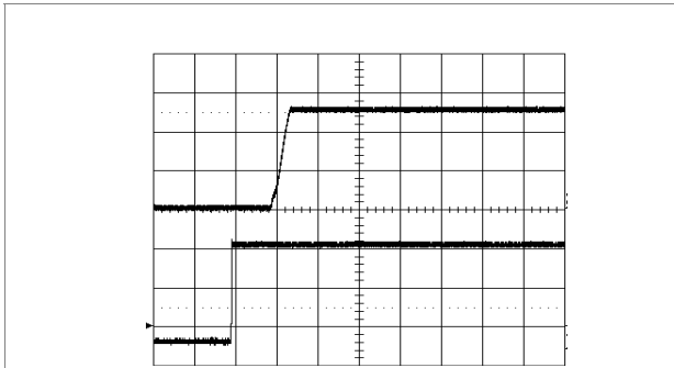
Start-up enabled by connecting V_i at: T_{ref} = +25^{\circ}\text{C} , I_o = 1.2\text{ A} resistive load, V_i = 53\text{ V} . Top trace: output voltage (1 V/div.). Bottom trace: input voltage (20 V/div.). Time scale: 2 ms/div.
