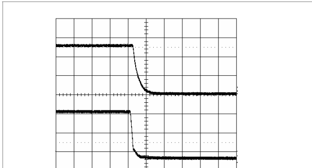
Shut-down enabled by disconnecting V_i at: T_{ref} = +25^{\circ}\text{C} , I_o = 1.2\text{ A} resistive load, V_i = 53\text{ V} . Top trace: output voltage (1 V/div.). Bottom trace: input voltage (20 V/div.). Time scale: 2 ms/div.
