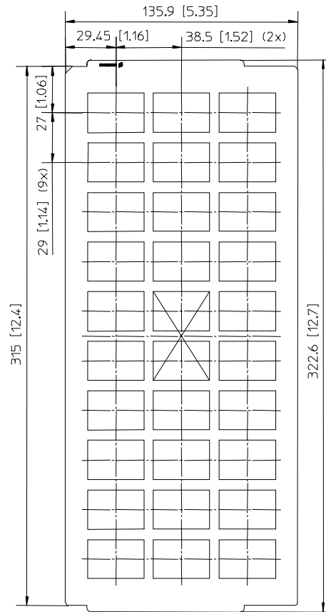
X = Vacuum pickup area.
