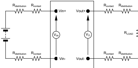
Figure 62. Output Ripple and Noise Test Setup.
