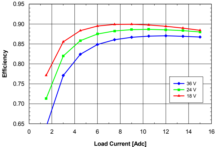
Fig. 3.3V.5: Efficiency vs. load current and input voltage for SQ24T/S15033 converter mounted vertically with air flowing from pin 3 to pin 1 at a rate of 300 LFM (1.5 m/s) and T_a = 25^\circ\text{C} .
