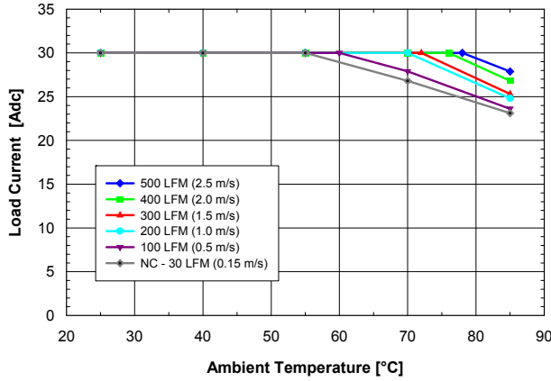
Fig. 1.5V.1: Available load current vs. ambient air temperature and airflow rates for SQE48T30015 converter mounted vertically with air flowing from pin 3 to pin 1, MOSFET temperature \leq 120^{\circ}\text{C} , V_{in} = 48\text{ V} .
