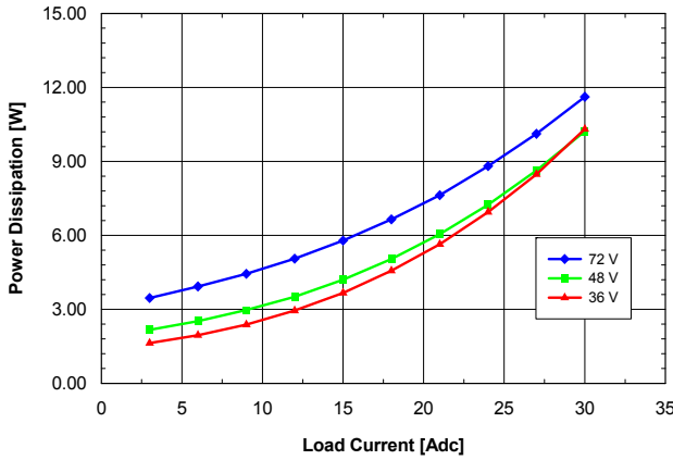
Fig. 3.3V.5: Power dissipation vs. load current and input voltage for SQE48T30033 converter mounted vertically with air flowing from pin 3 to pin 1 at a rate of 300 LFM (1.5 m/s) and T_a = 25\text{ }^\circ\text{C} .
