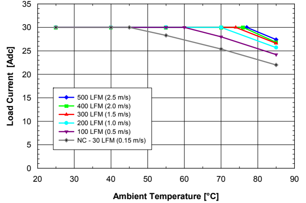
Fig. 1.5V.2: Available load current vs. ambient air temperature and airflow rates for SQE48T30015 converter mounted horizontally with air flowing from pin 3 to pin 1, MOSFET temperature \leq 120^{\circ}\text{C} , V_{in} = 48\text{ V} .
