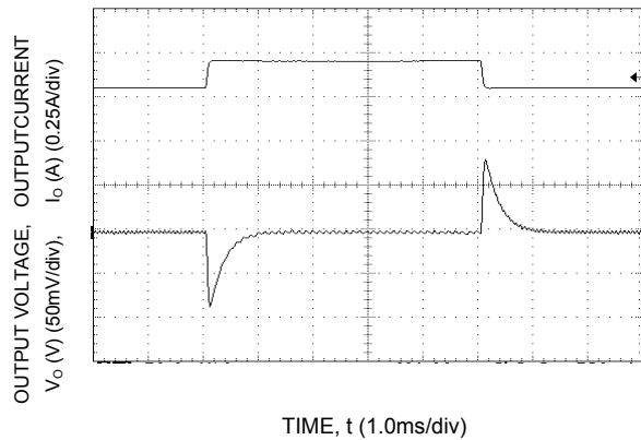
Figure 29. Transient Response to Dynamic Load Change from 50% to 75% to 50% of full load.
