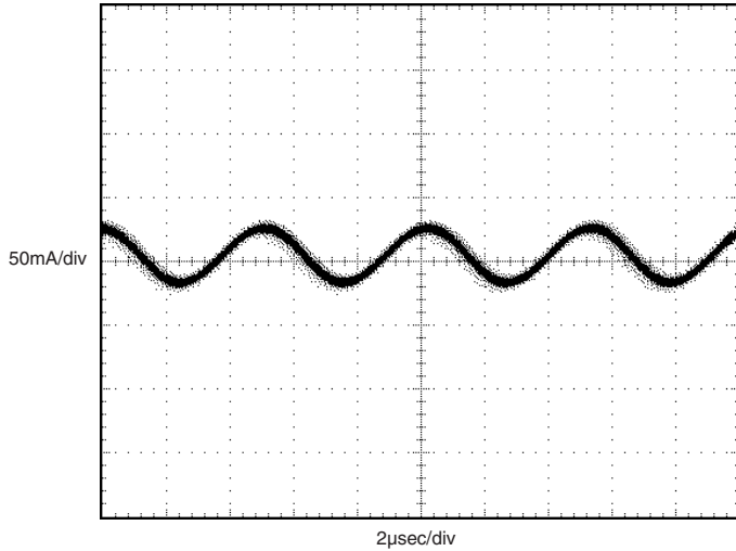
Input Reflected Ripple Current (Input Filter = 220µF/12µH/33µF, V IN = 12V, I OUT = 5V/10A)
