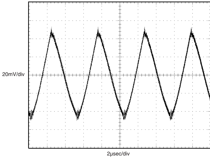
Output Ripple and Noise (V IN = 12V, V OUT = 5V/10A, C OUT = 22µF)
