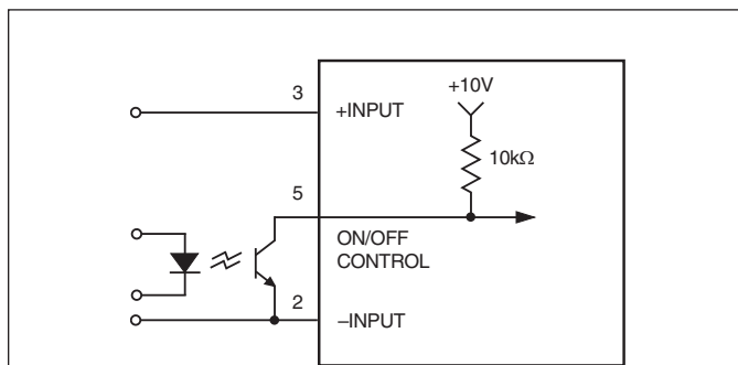
Figure 6. Driving the On/Off Control Pin
