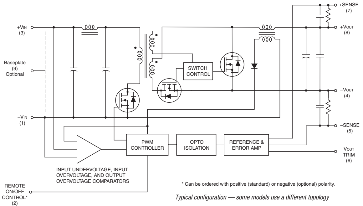
Figure 1. Simplified Schematic
