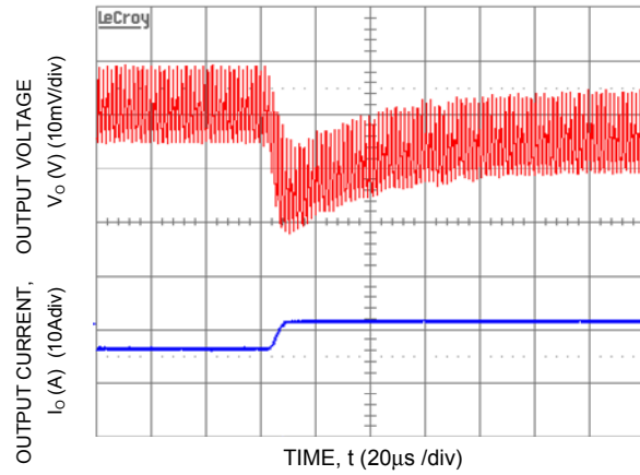
Figure 10. Transient Response to Dynamic Load Change from 50% to 100% at 12Vin, Cout-1x47µF+3x330µF, CTune-10nF & RTune-220ohms
