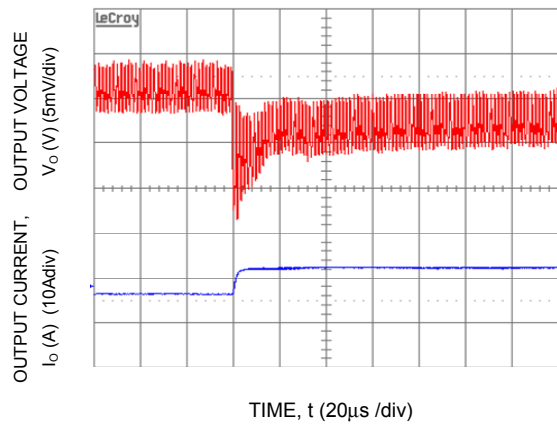
Figure 4. Transient Response to Dynamic Load Change from 50% to 100% at 12V in , C out -3x47µF+6x330µF, C Tune -47nF, R Tune -180ohms
