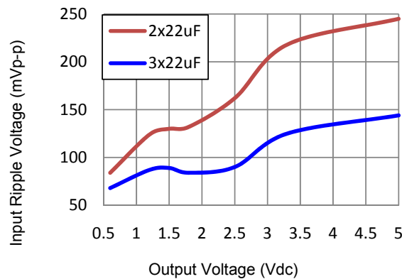
Figure 37. Input ripple voltage for various output voltages with 2x22 \mu\text{F} or 3x22 \mu\text{F} ceramic capacitors at the input (12A load). Input voltage is 12V.
