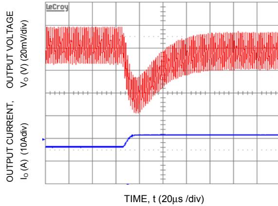
Figure 22. Transient Response to Dynamic Load Change from 50% to 100% at 12Vin, C_{out}=1 \times 47\mu\text{F} + 1 \times 330\mu\text{F} , C_{Tune}=330\text{pF} & R_{Tune}=270\text{ohms}
