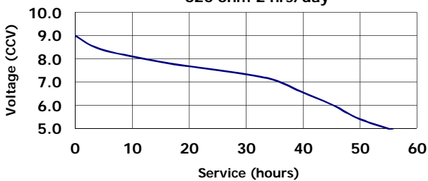
RADIO 620 ohm 2 hrs/day
