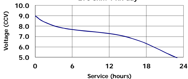
TOY 270 ohm 1 hr/day
