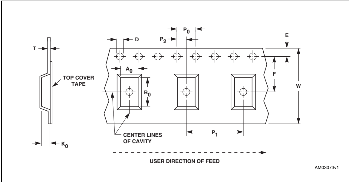
Figure 7. Carrier tape for SOT323-5L and UDFN-4L packages
