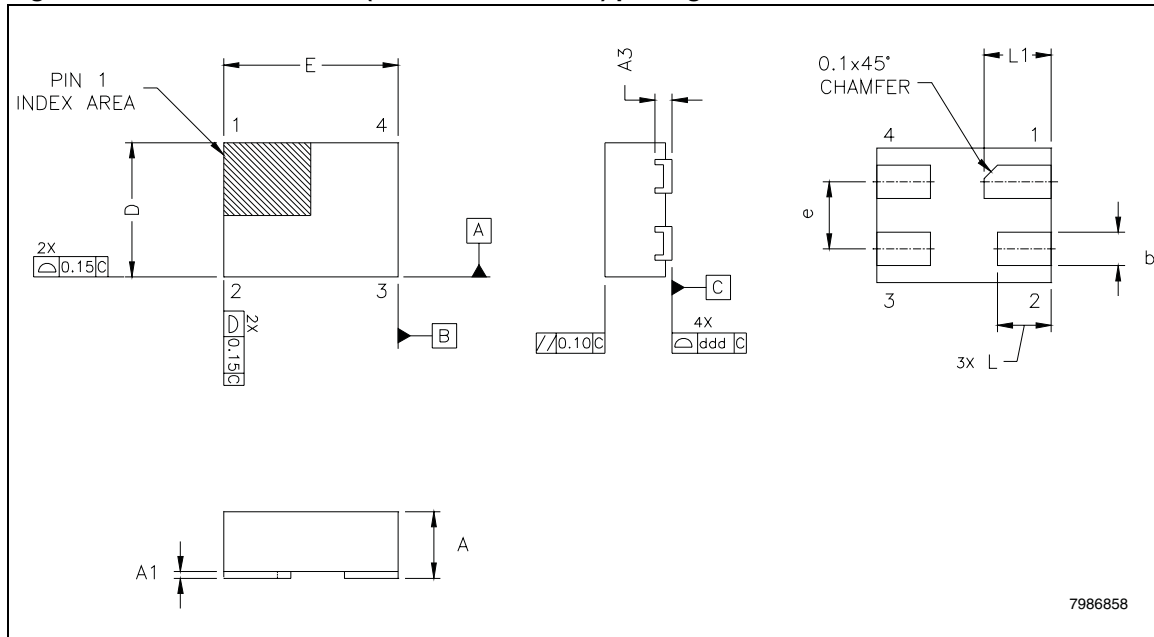
Figure 6. UDFN-4L – 4-lead (1.00 mm x 1.30 mm) package outline
