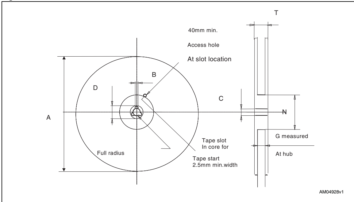
Figure 8. Reel schematic
