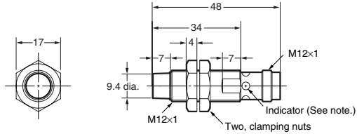
E2A-M12KN08-M1-□□/E2A-S12KN08-M1-□
