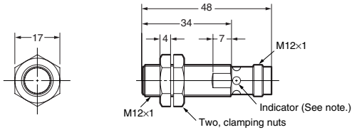
E2A-M12KS04-M1-□□/E2A-S12KS04-M1-□
