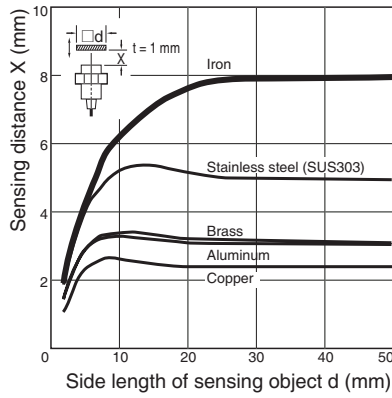
E2A-M12□N08/E2A-S12□N08
