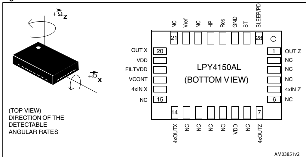
Figure 2. Pin connection
