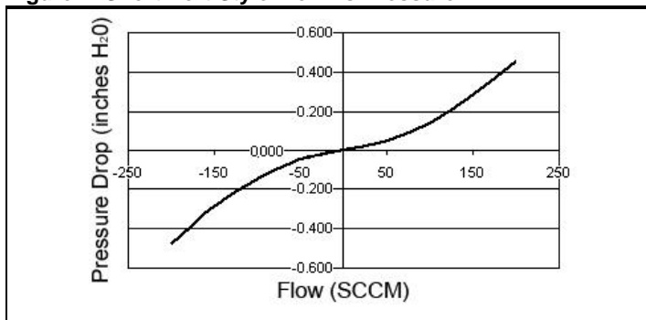
Figure 7 Short Port Style Flow vs Pressure
