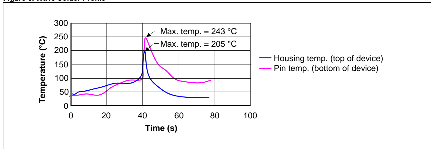
Figure 8. Wave Solder Profile
