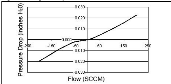
Figure 6. Long Port Style Flow vs Pressure
