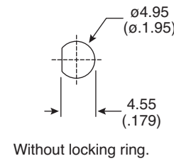
Panel Mounting
