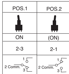
SWITCH FUNCTION
