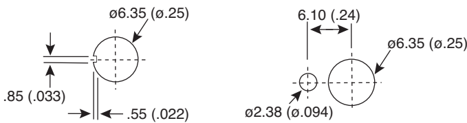
PANEL MOUNTING
