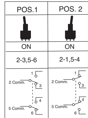
SWITCH FUNCTION
