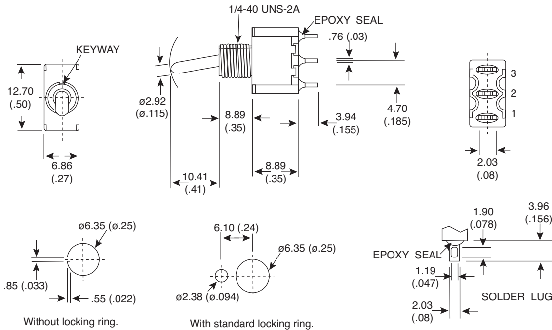
PANEL MOUNTING
