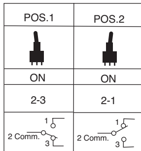
SWITCH FUNCTION
