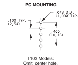
T101MH9V3BE SPDT
