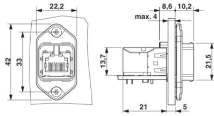
Push-Pull Anbaurahmen RJ45
