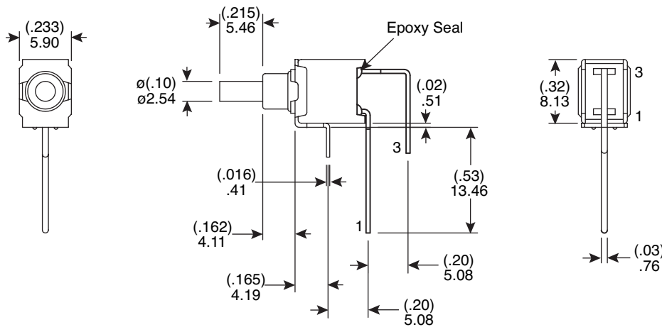
P.C. MOUNTING
