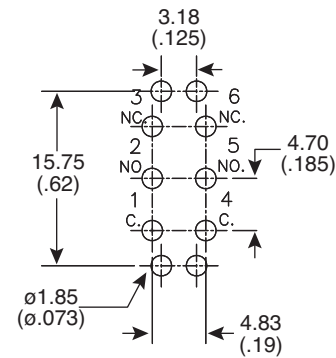
P.C. MOUNTING
