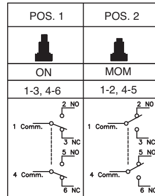
SWITCH FUNCTION
