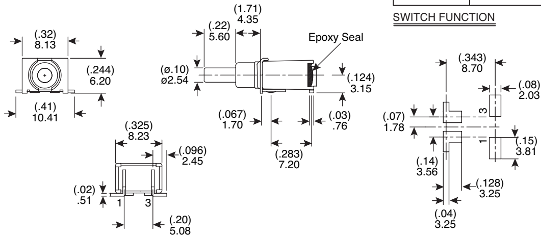
P.C. MOUNTING
