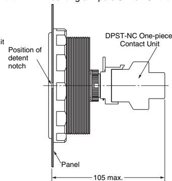
Mounting a 2-pole Switch Unit *
