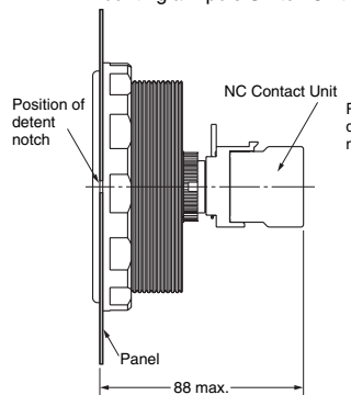
Mounting a 1-pole Switch Unit *
