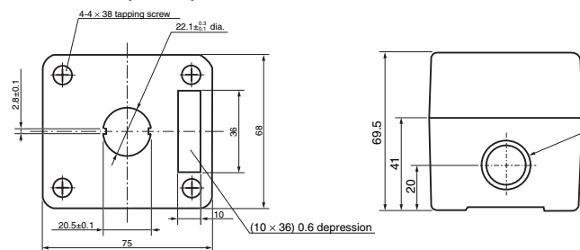
Control Box A22Z-B101Y (1 hole)
