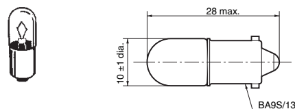
Incandescent Lamp A22-5, 12, 24, H1
