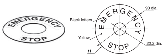
Lock Ring A22Z-3360
