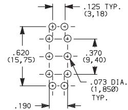
8261SH9_BE2 DPDT
