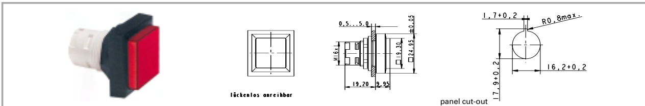
panel cut-out
