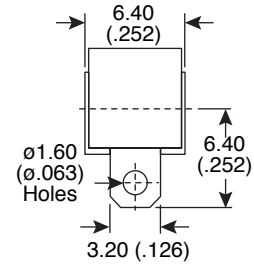
Solder Terminal
