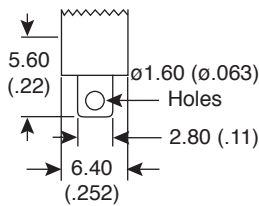
Solder Terminals
