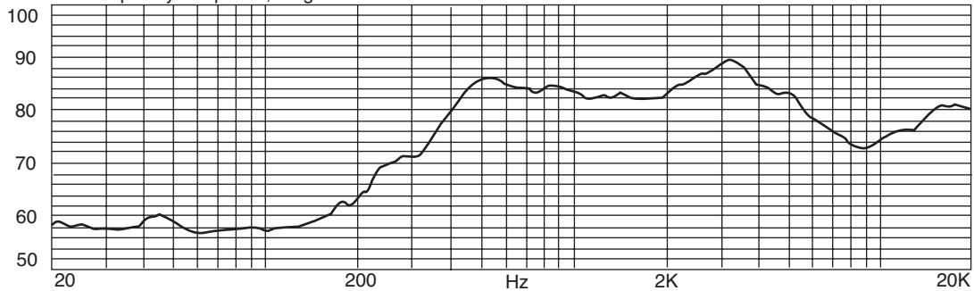
A: Frequency Response, Magn dB re 20.00PA
