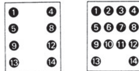
Terminal Arrangement (Bottom View)
