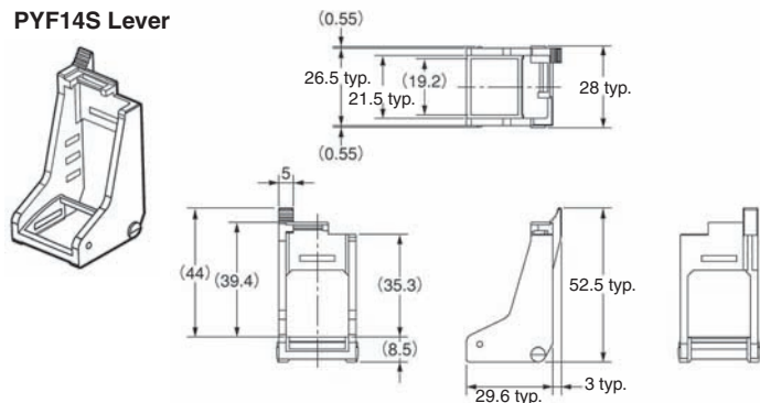
PYF14S Lever
