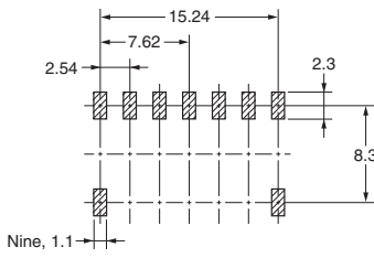
Mounting Dimensions (Top View) Tolerance: \pm 0.1 mm
