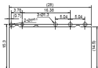
PC board mounting hole layout (BOTTOM VIEW)
