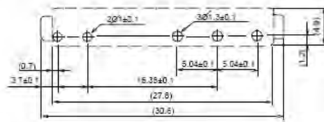
PC Board Mounting Hole Layout (BOTTOM VIEW)
