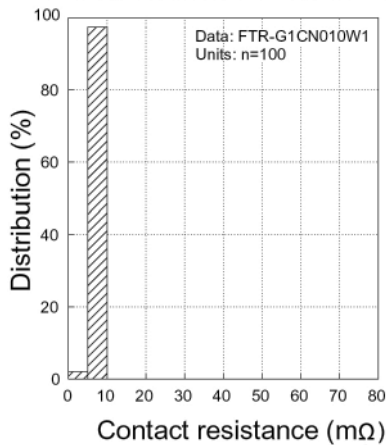
Contact resistance distribution
