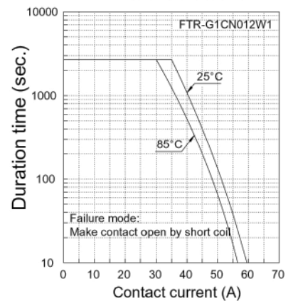
Contact current
