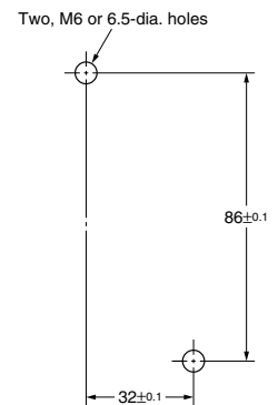
Mounting Hole Dimensions (TOP VIEW)
