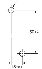
Mounting Hole Dimensions (TOP VIEW)
