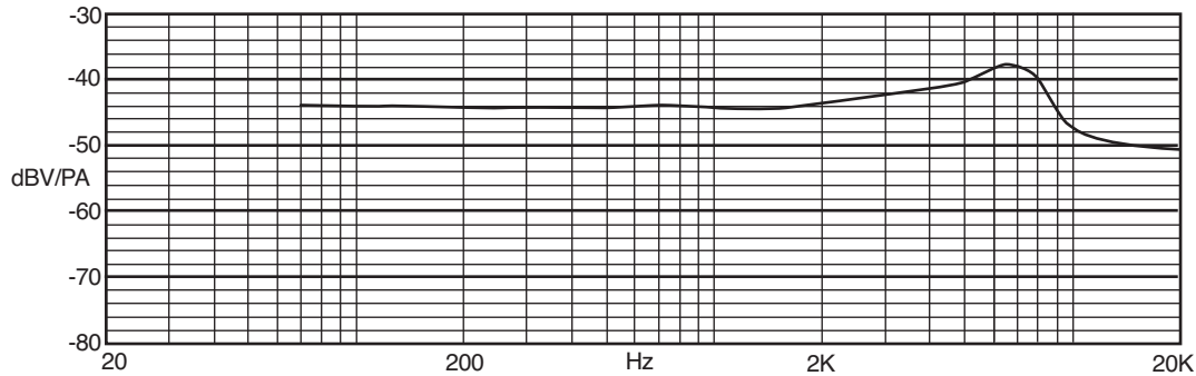
Microphone Frequency Response
