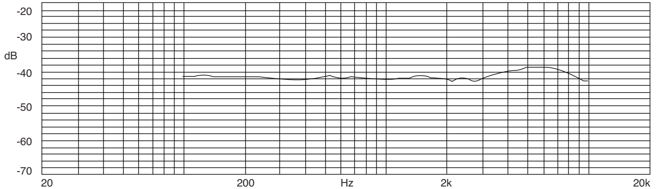
A: Frequency Response, Magn dB Ref. 1V/Pa
