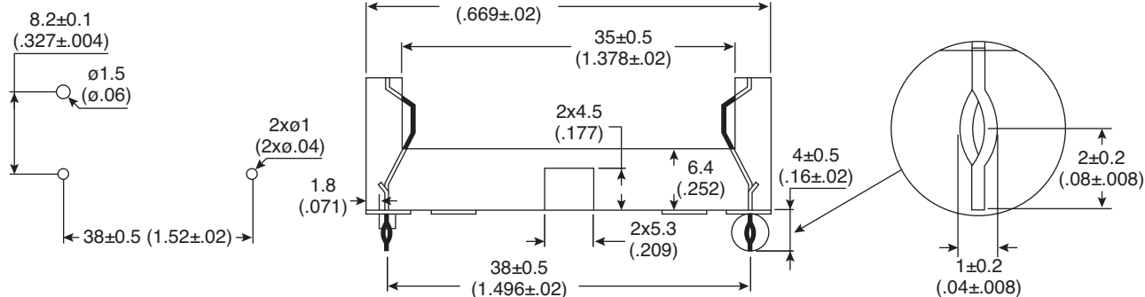
PCB/Mounting Layout
