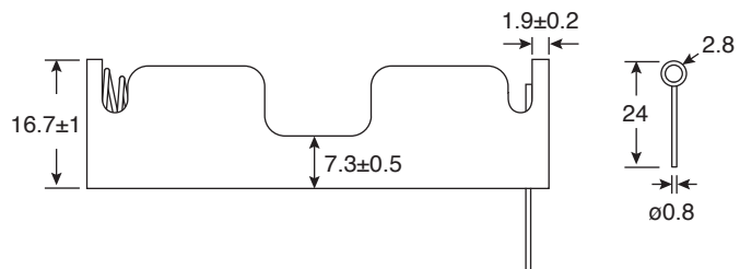
Dimensions: mm
