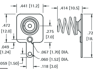
DUAL CONTACTS WITH TAB
