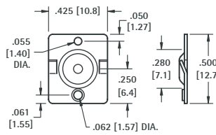
(+) POSITIVE BUTTON
