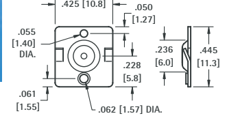
(+) POSITIVE BUTTON
