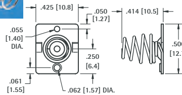
CAT. NO. 5222
