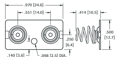
DUAL SPRING CONTACT
