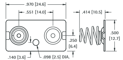
DUAL CONTACTS
