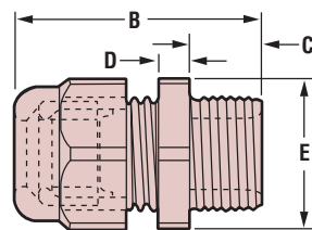
SEALING NUT
